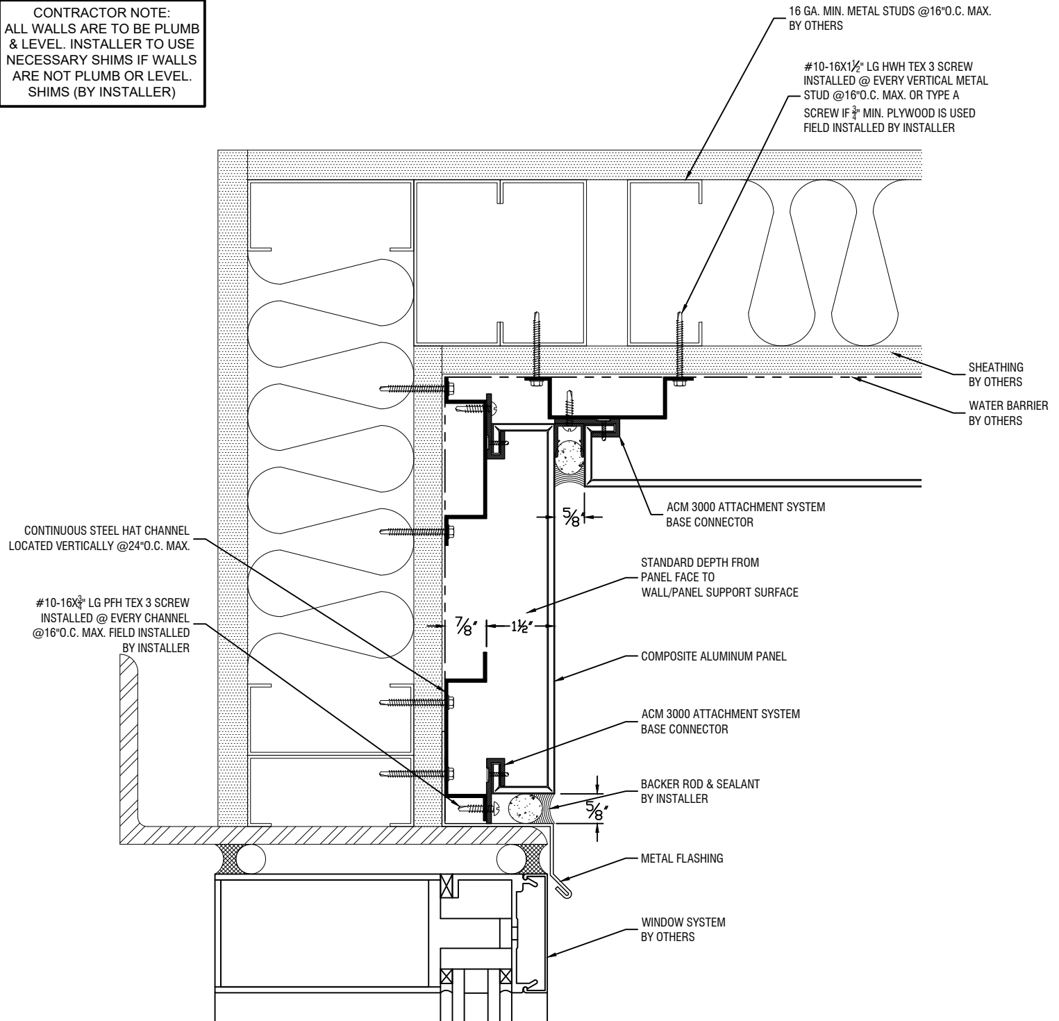
Canopy Detail
