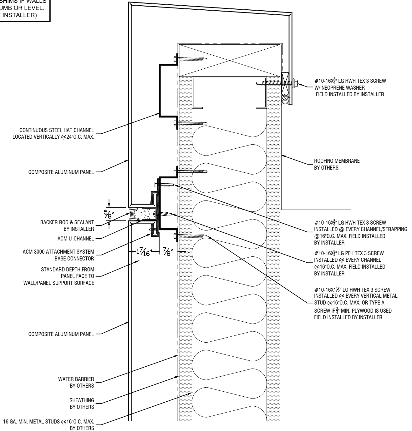
Coping Detail-2
