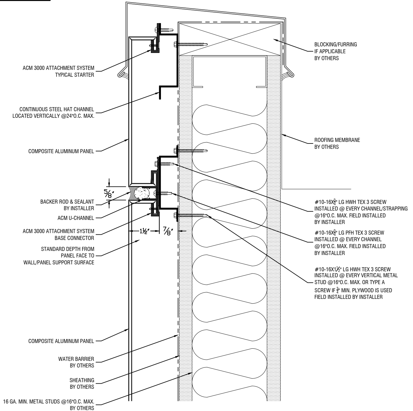
Coping Detail-1
