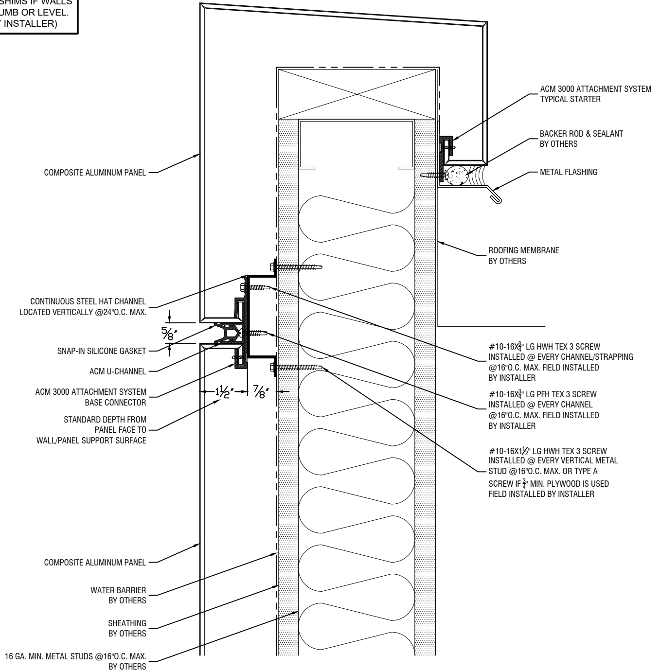
Coping Detail-2
