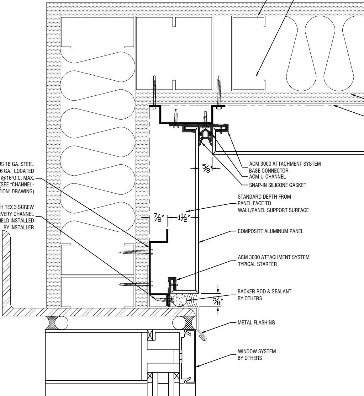
Canopy Detail
